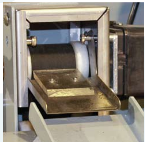
Belt skimmer for removal of oils and greases
